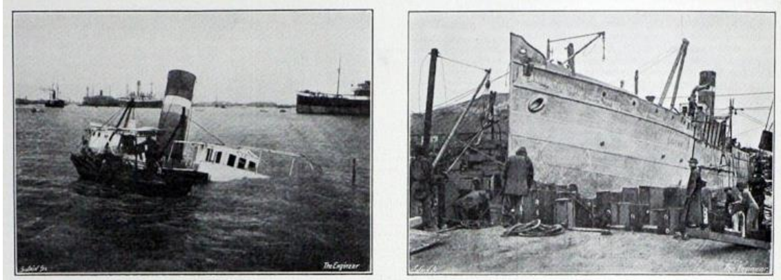
US Army Transport LISCUM ex KONGSEE sunk at Shanghai, Sept. 1913 and subsequently docked for repair, masts removed ( The Engineer ).
