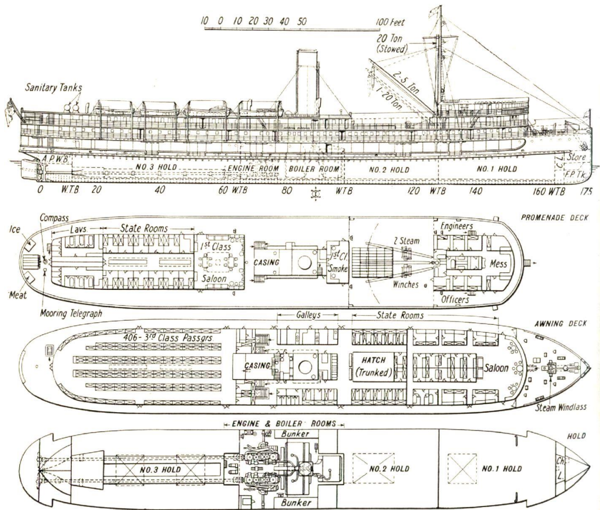
KUNG WO Largest river steamer on the Yangtze ( Shipping Wonders of the World ).
