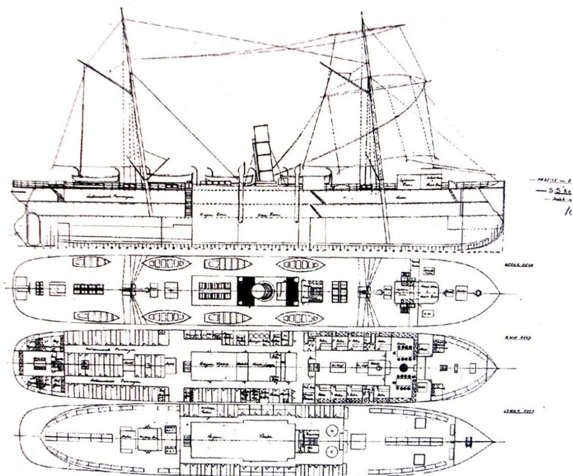
VICKERS ARMSTRONG COLLECTION YARD No. 104. S.S. KOW-SING (1883). For INDO-CHINA STEAM NAVIGATION Co. LTD. LONG
