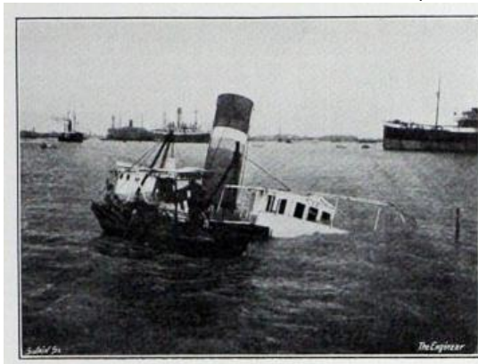
US Army Transport LISCUM ex KONGSEE sunk at Shanghai, Sept. 1913 and subsequently docked for repair, masts removed ( The Engineer ).
