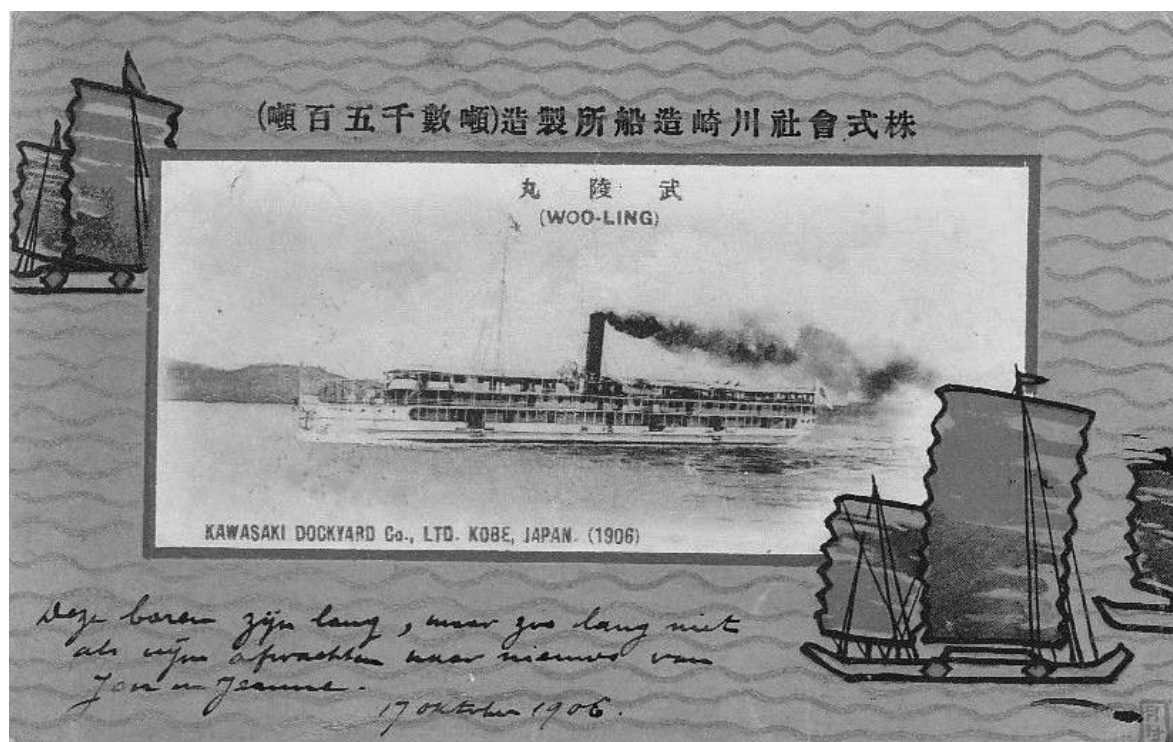
1906 Kawasaki Zosen postcard depicting WOO-LING MARU trials off Kobe, bridge deck superstructure extending to funnel and low freeboard (Internet).
