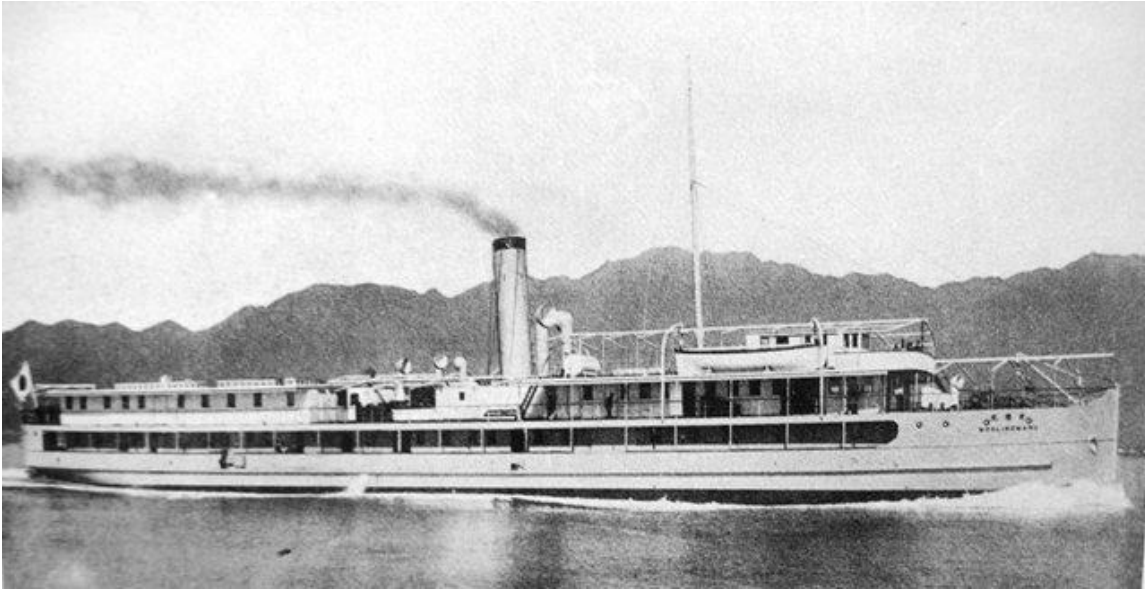
Final WOO-LING MARU trials off Kobe in Hunan Kisen colours with shorter bridge deck, greater freeboard, and large lifeboat (builders).
