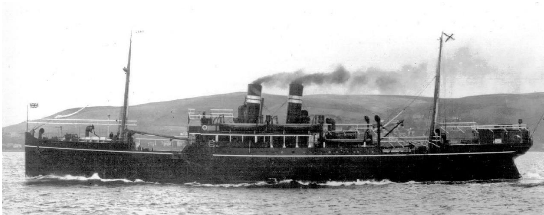
Turbine steamer LAMA during trials on the Clyde on completion for B.I. (WSPL).
