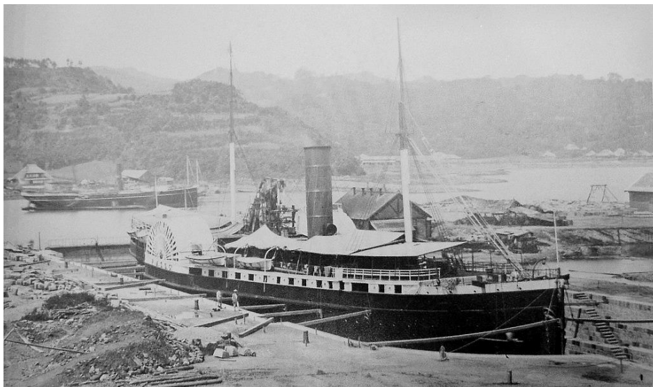
Identified as OREGONIAN in Yokosuka No.1 dydock (Verny coll.).
