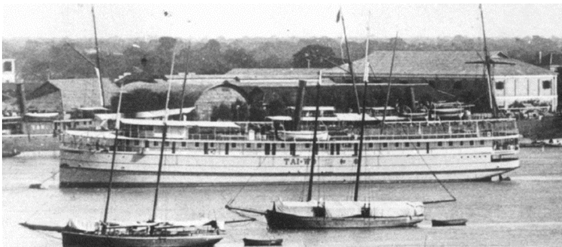
TAI WO at Shanghai, top deck built up aft (JM&C (from a Kung Tai panorama)).
