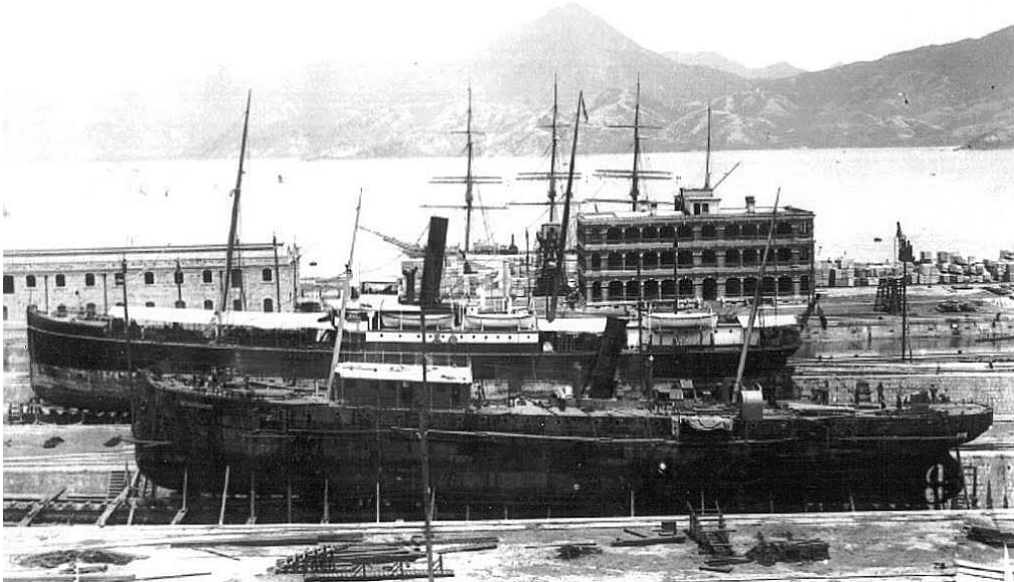
PEDRO DE SOTOLONGO at Taikoo Dockyard 2010 after lengthening and plating in of the well deck but prior to renaming as UNION, CNC's Nanchang on other side (HKMM).
